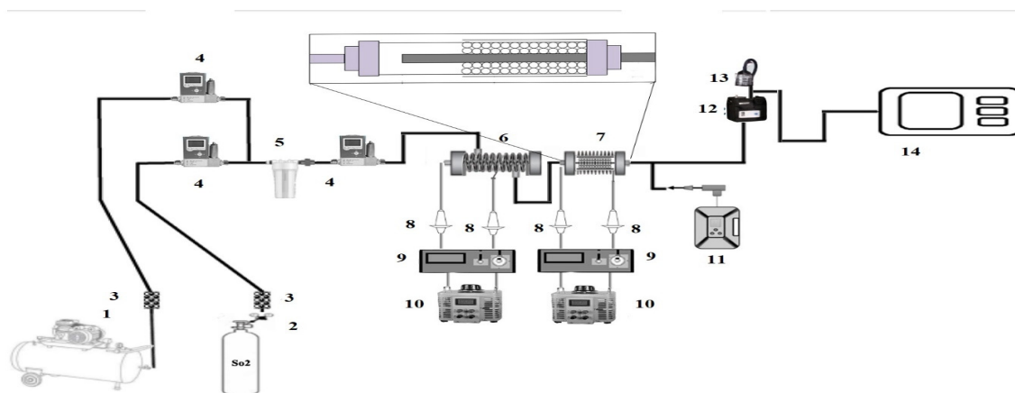
Fig. 1. Schematic diagram of the cold plasma device (DBD) setup for SO 2 removal. 1. Compressor 2. SO 2 Cylinder 3. Silica Gel 4. Mass Flow Controller (MFC) 5. Mix Chamber 6. Reactor 1 7. Reactor 2 8. High Voltage Probe 9. High Voltage Power Supply 10. Variac 11. Testo 350 12. Personal Sampling Pump 13. Cassette and filter 14. Ion chromatography
